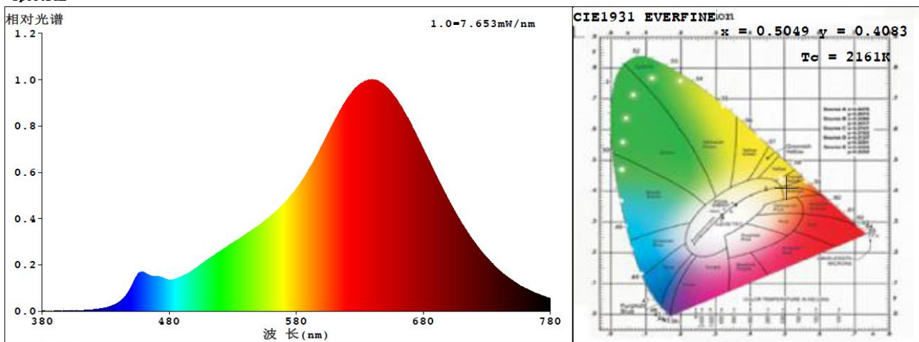
Spectral Distribution
